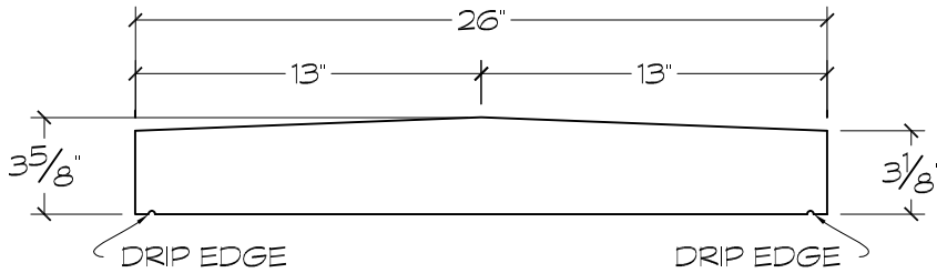
CROSS SECTION
